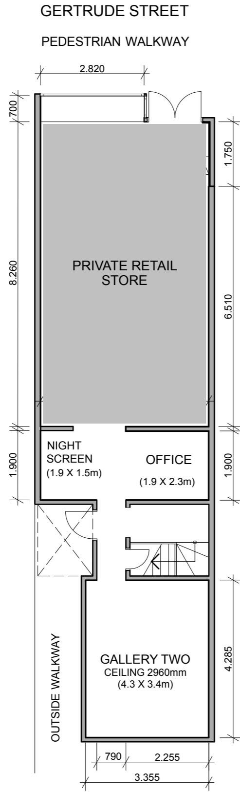
GROUND FLOOR PLAN SCALE 1:100 @ A3
